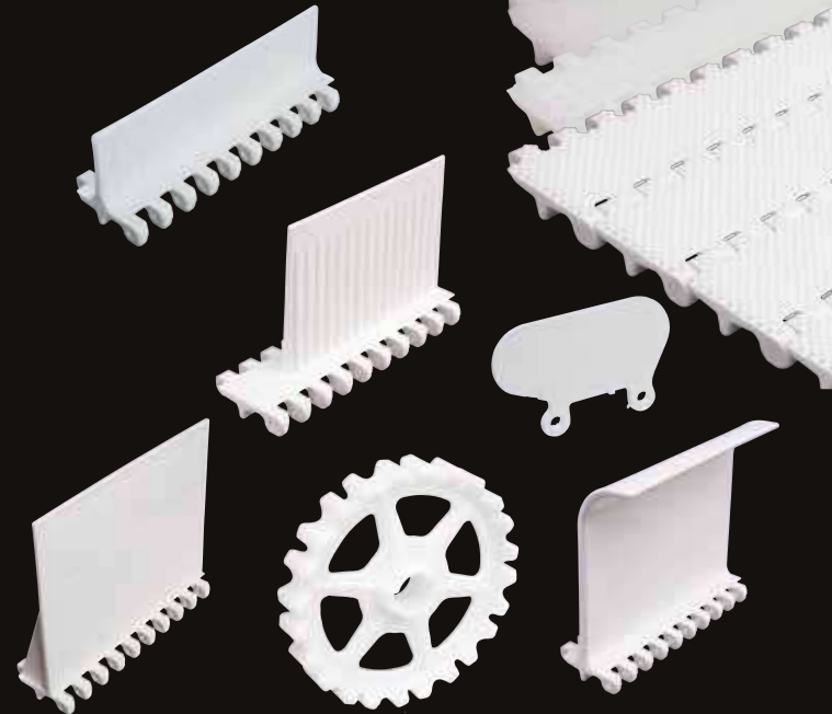
50-808 Flat top closed surface. EASY TO CLEAN food applications.
